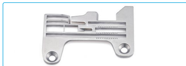
名称: 针板(厚料) Description: Needle Plate (Heavy Duty) 代码/Part NO: 20715050 适配: E4/JK-798TDI Machine Type: E4/JK-798TDI
