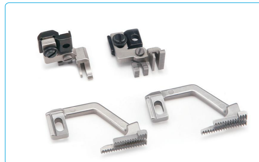
名称: 送料组件 Description: Feed Assy 代码/Part NO: 2011401800 适配: E3-3-M1-15 Machine Type: E3-3-M1-15
