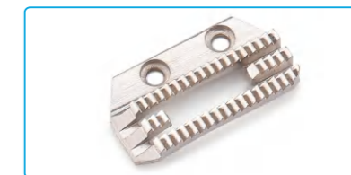
名称: 送料牙 Description: Feed Dog 代码/Part NO: 11314001 适配: 平缝机"-H"机型 (除A6F外) Machine Type: Lockstitch"-H" model (Except "A6F")
