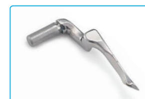
名 称: 上弯针 Description: Upper Looper 代 码/Part NO: 20717050 适 配: E4/C3/C4/C5/798T系列H/M和A04/435机型 Machine Type: H/M/A04/435 type for E4/C3/C4/C5/798T series
