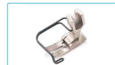
名称: 短距缝带刀压脚组件 Description: Presser Foot With Knife (Short Distance Sewing) 代码/Part NO: 1411600400 适配: 平缝带“-N”机型 Machine Type: A5-WN, A4S-N
