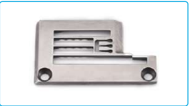
名称: 针板(356) Description: Needle Plate (356) 代码/Part NO: 30115045 适配: W4/W4S系列-23BB机型 Machine Type: 23BB type for W4/W4S series
