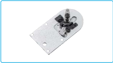
名称: 针板组件 Description: Needle Plate Asm. 代码/Part NO: 4031560100 适配: JK-T1900G/1906G Machine Type: JK-T1900G/1906G
