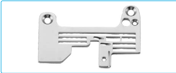
名称: 针板(包兜机) Description: NEEDLE PLATE 代码/Part NO: 121115005 适配: C5/C5F/C6-02×250 Machine Type: C5/C5F/C6-02×250
