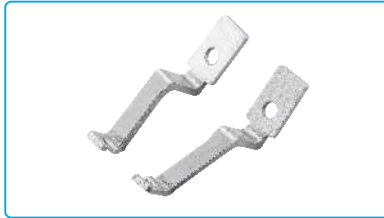
名称: 压脚组件 Description: Presser Foot Assy. 代 码/Part NO: 140316012+140316011 适 配: JK-T1900G Machine Type: JK-T1900G
