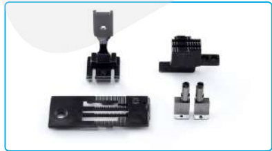
名称: 针位(1/2) Description: Needle Gauge 1/2 代 码/Part NO: 810592+12915312 适 配: JK-58450G/J 58750G/J Machine Type: JK-58450G/J 58750G/J
