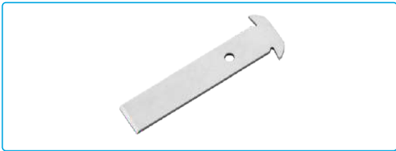
名称: 面线动刀14-16mm Description: Upper Movable Knife 14-16mm 代 码/Part NO: 42119005 适 配: JK-T5878-68/78 Machine Type: JK-T5878-68/78
