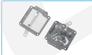
名称: 针板组件 Description: NEEDLE PLATE ASM. 代码/Part NO: 4131500600 适配: JK-T1790BK/1791BK/1792BK/ 1791GK/1792GK Machine Type: JK-T1790BK/1791BK/1792BK/ 1791GK/1792GK
