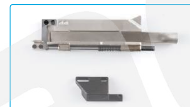
名称: 自动剪线刀组件 Description: Thread Trimmer Asm 代码/Part NO: 2071208900 适配: C4/C5-BK Machine Type: C4/C5-BK
