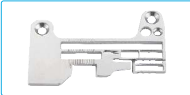
名称: 针板(5线厚料) Description: Needle Plate (H) 代码/Part NO: 121115003 适配: C5F/C6/C7系列M04/435机型 Machine Type: M04/435 type of C5F/C6/C7 series
