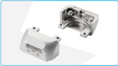
名称: 单针针板组件(中孔) Description: Needle Plate Asm.(M) 代 码/Part NO: 15521500100 适 配: S5-91/S7-91 Machine Type: S5-91/S7-91
