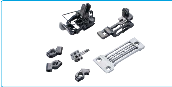
名称: 针位组件(1/8) Description: Needle Gauge Set (1/8) 代 码/Part NO: 4063402000 适 配: JK-T9280D-73(1/8) Machine Type: JK-T9280D-73(1/8)
