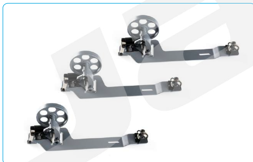
名称: 绕线器组件 Description: Bobbin Winder 代码/Part NO: 1163101600 适配: JK-609S Machine Type: JK-609S
