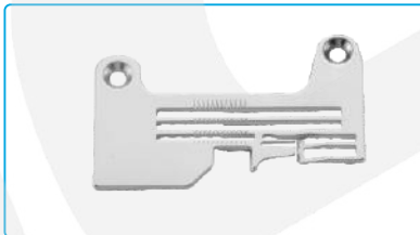
名称: 四线针板 Description: NEEDLE PLATE 代码/Part NO: 21315201 适配: C5/C5S/C8-4 Machine Type: C5/C5S/C8-4
