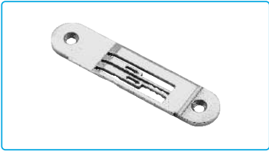
名称: 斜双针针板 (3/16) Description: Needle Plate(3/16) 代 码/Part NO: 12515010 适 配: JK-8558G/JK-8558WD-1 (3/16) Machine Type: JK-8558G/JK-8558WD-1(3/16)
