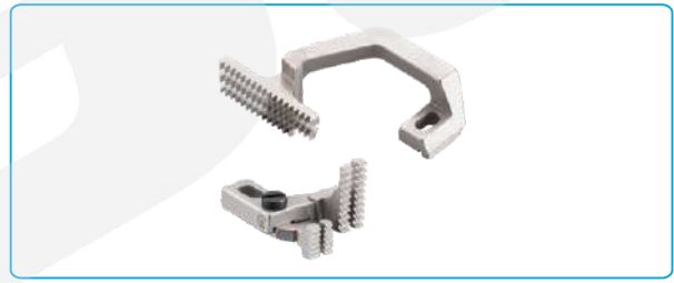
名称: C5F-2567送布牙组件 Description: Feed Dog 代 码/Part NO: 12111404200 适 配: C5F-A/C7-4-M03/333/C5F-A-3-02/233 Machine Type: C5F-A/C7-4-M03/333/C5F-A-3-02/233
