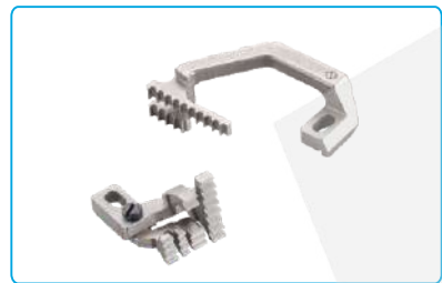
名称: 牙齿组件 Description: Feed Dog 代 码/Part NO: 12131400600 适 配: C2/C4/C5/C5F/C6/E4S/C7系列M04/435机型 Machine Type: M04/435 type of C2/C4/C5/C5F/C6/E4S/C7 series
