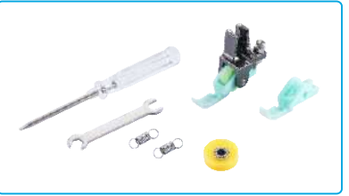
名称: T36LN 滚轮款 天蓝底+柠檬齿轮 配胶轮 (6件套) Description: T36LN roller press foot(6-piece set) 代码/Part NO: 813901 适配: 平缝机通用 Machine Type: All locktitch machine series
