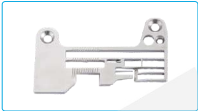
名称: 针板(六线厚料) Description: Needle Plate (6-thread, H) 代码/Part NO: 121115002 适配: C5F/C6/C5S/C7系列M04/435机型 Machine Type: M04/435 type of C5F/C6/C5S/C7 series
