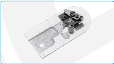
名称: 针板组件 Description: Needle Plate Asm. 代码/Part NO: 4231500300 适配: JK-T1904BS/JK-T1906BS Machine Type: JK-T1904BS/JK-T1906BS
