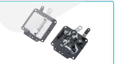
名称: 针板组件 Description: NEEDLE PLATE ASM. 代码/Part NO: 4131500800 适配: JK-T1790GS/JK-T1791GS/JK-T1792GS Machine Type: JK-T1790GS/JK-T1791GS/JK-T1792GS
