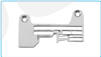
名称: 毛巾机针板 Description: NEEDLE PLATE 代码/Part NO: 121115021 适配: C4-6-M54/435/X Machine Type: C4-6-M54/435/X
