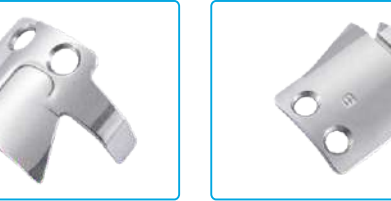
名称: 活动刀(厚料短槽) Description: Movable Knife 代 码/Part NO: 114119002 适 配: A2-CH/A2B-CH/A2C-CH/A3E-CH/A4B-CH/A4F-H/A5E-H/A7-DH Machine Type: A2-CH/A2B-CH/A2C-CH/A3E-CH/A4B-CH/A4F-H/A5E-H/A7-DH
