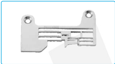
名称: 毛巾机针板 Description: NEEDLE PLATE 代码/Part NO: 20715088 适配: C4-6-53/233, C4MJ-4-53/233, C5FMJ-4-53/233 Machine Type: C4-6-53/233, C4MJ-4-53/233, C5FMJ-4-53/233
