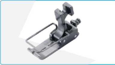
名称: 单针压脚 Description: Single-needle Presser Foot 代 码/Part NO: 1251601000 适 配: JK-8558G-1/JK-8558WD-2 Machine Type: JK-8558G-1/JK-8558WD-2
