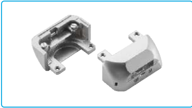
名称: 单针针板组件(大孔) Description: NEEDLE PLATE (L) 代 码/Part NO: 15521505100 适 配: JK-6671C-H/S5-91-H/S7-91-H Machine Type: JK-6671C-H/S5-91-H/S7-91-H
