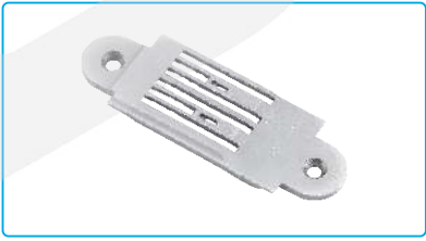
名称: 斜双针针板 (1/2) Description: Needle Plate(1/2) 代 码/Part NO: 12515015 适 配: JK-8558G/JK-8558WD-1 (1/2) Machine Type: JK-8558G/JK-8558WD-1(1/2)
