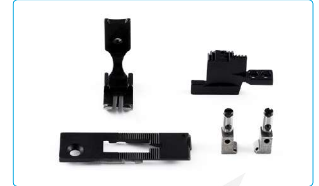
名称: 针位(1/8) Description: Needle Gauge 1/8 代 码/Part NO: 810590+12915306 适 配: JK-58450G/J 58750G/J Machine Type: JK-58450G/J 58750G/J
