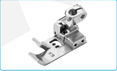
名称: 压脚 (35AC, 364) Description: Presser Foot(35AC, 364) 代码/Part NO: 30216008 适配: JK-8669/K4/K5/K5E/K6A-35ACx364 Machine Type: JK-8669/K4/K5/K5E/K6A-35ACx364
