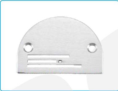
名称: B型三排针板16 Description: Needle Plate B16 代 码/Part NO: 812757 适 配: 平缝系列 Machine Type: Lockstitch Machine Series
