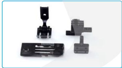
名称: 针位(1/2) Description: Needle Gauge 1/2 代 码/Part NO: 810588+12915312 适 配: JK-58420G/J 58720G/J Machine Type: JK-58420G/J 58720G/J
