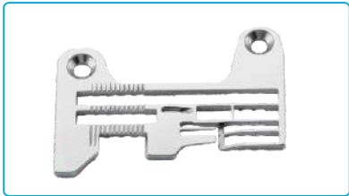
名称: 针板(六线厚料) Description: Needle Plate (6-thread, H) 代码/Part NO: 121215003 适配: JK-798TDI/E4/E4S-6-M04/435 Machine Type: JK-798TDI/E4/E4S-6-M04/435
