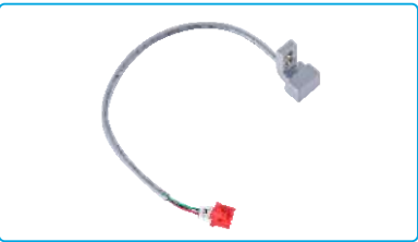
名称: 霍尔组件 Description: Sensor 代 码/Part NO: 2113003200 适 配: C5F/C7-02×250,C5/C6/C8, C7-BK, C5F-BK ,C5S-BK Machine Type: C5F/C7-02×250,C5/C6/C8, C7-BK, C5F-BK ,C5S-BK
