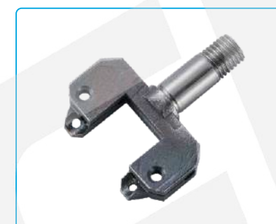
名称: 针夹头14mm Description: Needle Clamp 14mm 代 码/Part NO: 42134021 适 配: JK-T5878-68 Machine Type: JK-T5878-68
