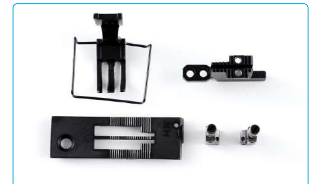
名称: 送布牙1/4(-5) Description: Needle Gauge 1/4 (-5) 代 码/Part NO: 11734003+11734002+12914314 +12915206+1291632500 适 配: JK-58450G/J-405 58750G/J-405 Machine Type: JK-58450G/J-405 58750G/J-405
