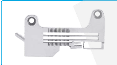
名称: 针板 Description: Needle Plate 代码/Part NO: 120015005 适配: C5-4-83/323/BK Machine Type: C5-4-83/323/BK
