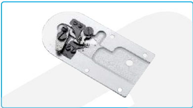
名称: 针板组件 Description: Needle Plate Asm. 代码/Part NO: 4031501500 适配: JK-T1900AH/1900BH Machine Type: JK-T1900AH/1900BH
