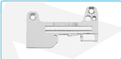
名称: 针板(三线卷边缝) Description: NEEDLE PLATE 代码/Part NO: 21115209 适配: C5/C5S/C5F/C6-3-32R2/223 Machine Type: C5/C5S/C5F/C6-3-32R2/223
