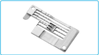
名称: 针板 (35AC, 364) Description: NEEDLE PLATE(35AC, 364) 代码/Part NO: 30215027 适配: JK-8669-35ACx364 Machine Type: JK-8669-35ACx364
