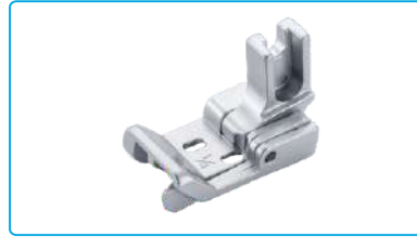
名称: 斜双针压脚 (1/4) Description: 2-Needle Presser Foot (1/4) 代 码/Part NO: 1251600100 适 配: JK-8558G/JK-8558WD-1 (1/4) Machine Type: JK-8558G/JK-8558WD-1 (1/4)
