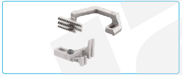
名称: C6-0911送布牙组件 Description: Feed Dog 代 码/Part NO: 2131400100 适 配: C2/C3/C4/C5F/C6/C8/E4S/798T系列M03/333机型 Machine Type: M03/333 type of C2/C3/C4/C5F/C6/C8/E4S/798T series
