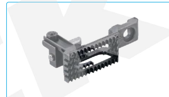
名称: 送料牙 (1/4) Description: FEED DOG(1/4) 代码/Part NO: 40614007 适配: JK-T9280 Machine Type: JK-T9280
